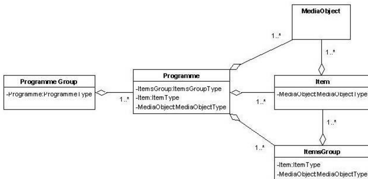
Figure 2: rough content structure around which P_META has been built
